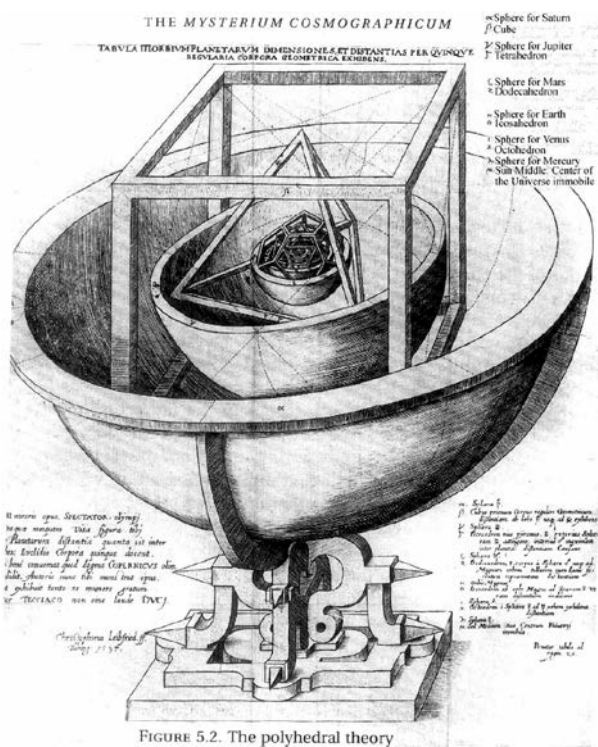
FIGURE 5.2. The polyhedral theory
